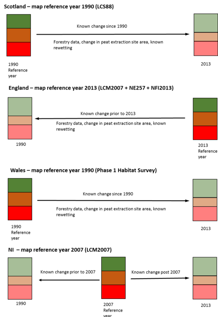
Figure 3.6. Schematic illustration of the approach used to derive activity data for emissions accounting in each UK country. The map reference year (for which full mapped condition data were derived) is shown in bold colours, different colours at each time point represent different peat condition categories. For illustrative purposes only three categories are shown rather than the 16 for considered in this project. Changes relative to the reference year (since the 1990 inventory baseline year and/or up to the present) were estimated from information on peat restoration projects and other land-cover changes (see Section 3.3).
